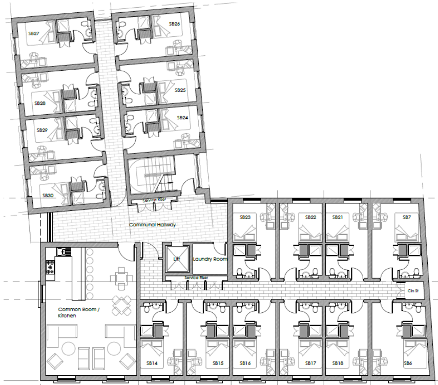
Indicative Second Floor Layout (17 Bedrooms)
